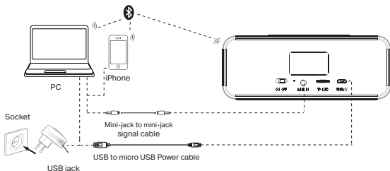
Fig. 4. Connection diagram
